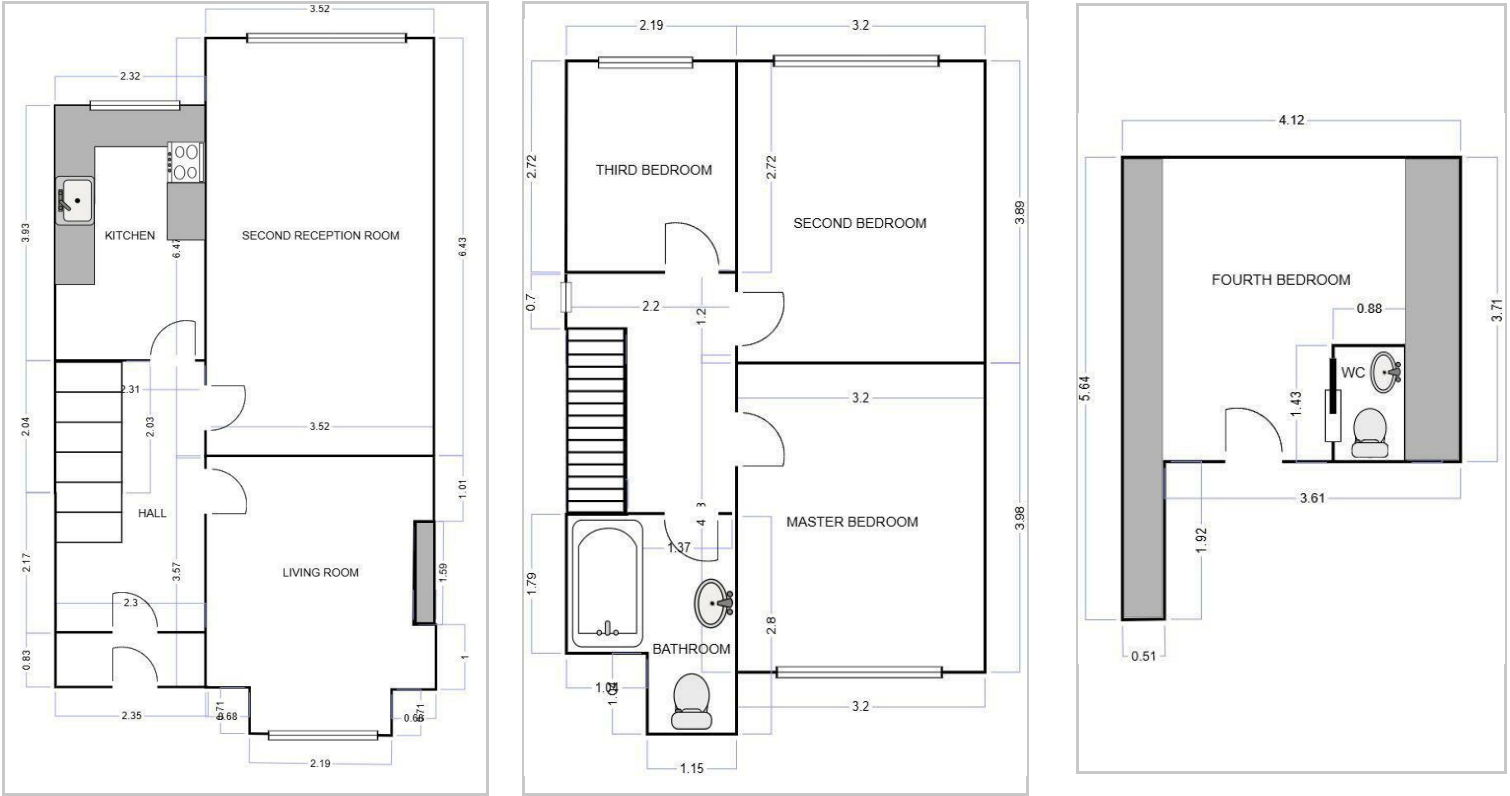
Floor Plan
