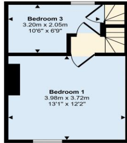
First Floor Approx 24 sq m / 253 sq ft
