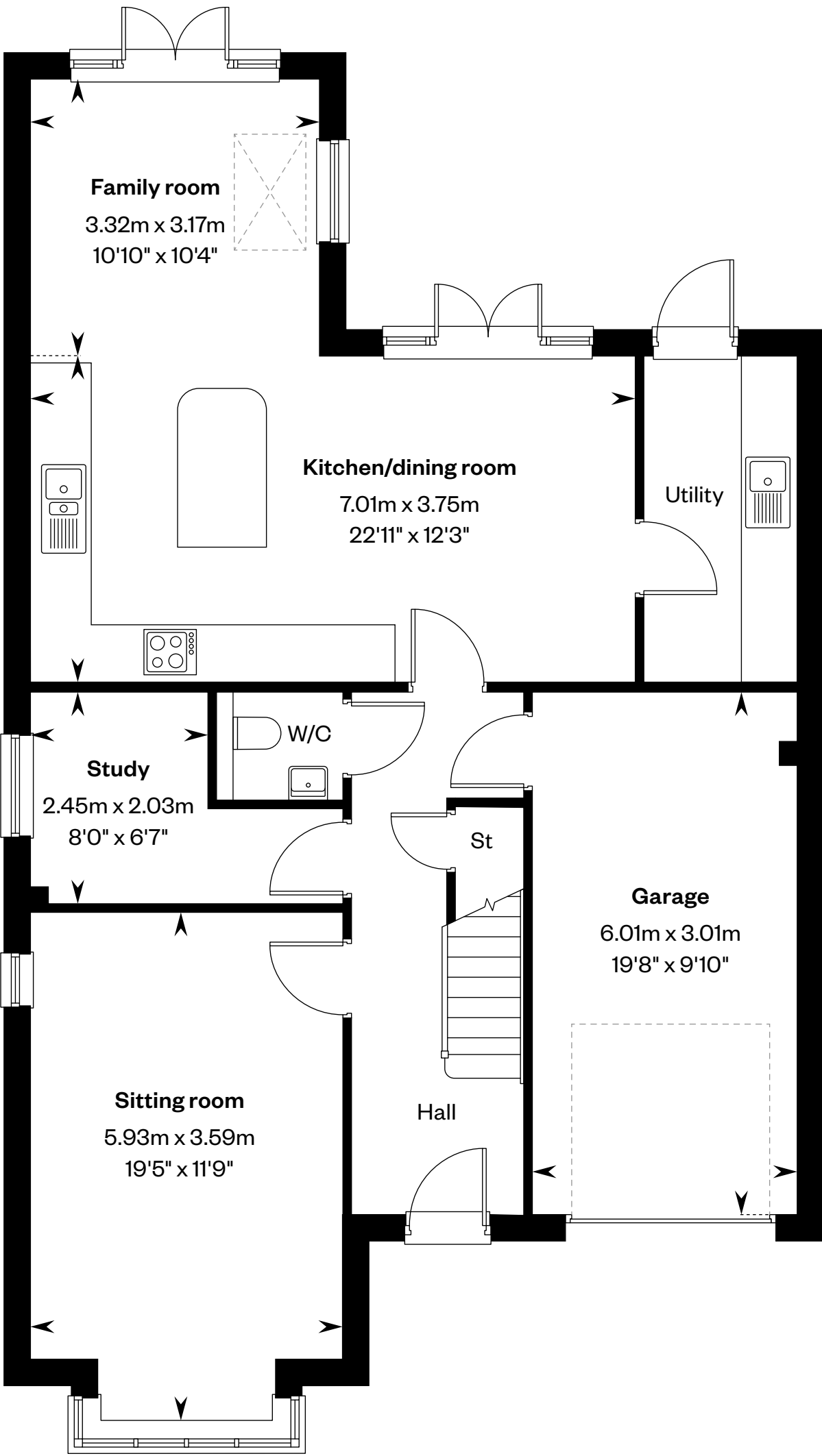
Ground floor
