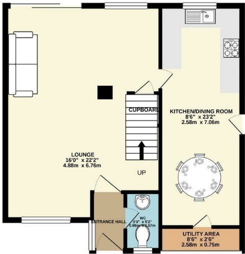
GROUND FLOOR 590 sq.ft. (54.8 sq.m.) approx.
