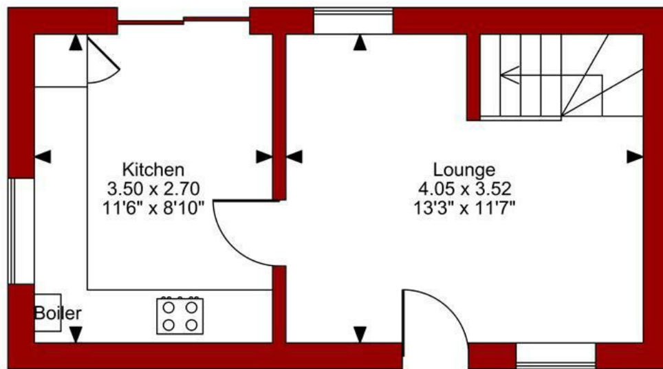
Ground Floor
