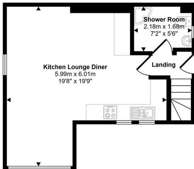
First Floor Approx 34 sq m / 366 sq ft
