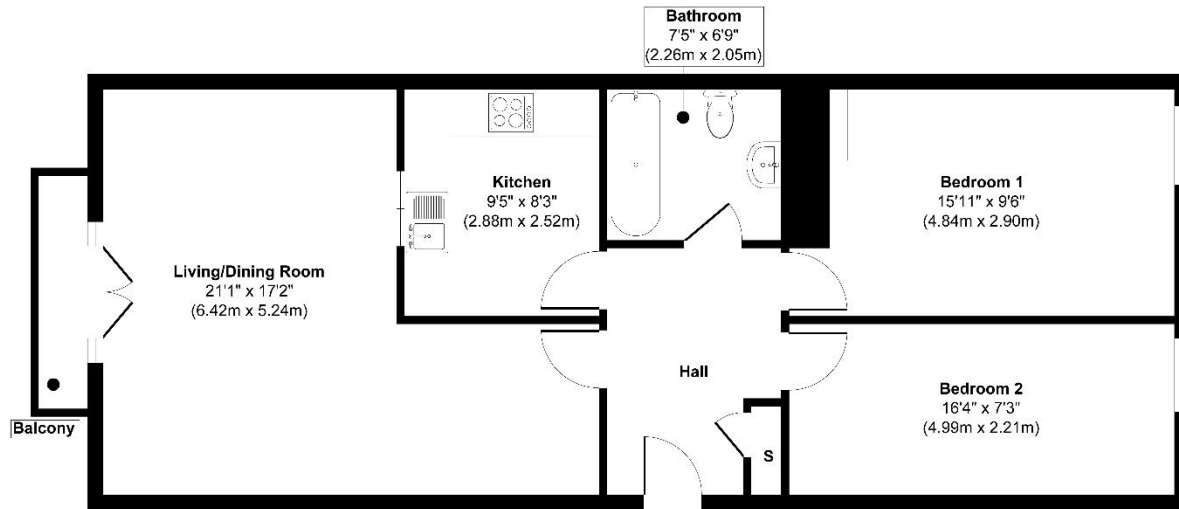
Floor Plan
