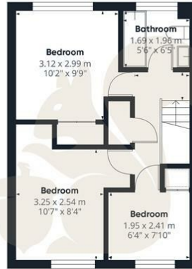
Floor 1 Building 1
