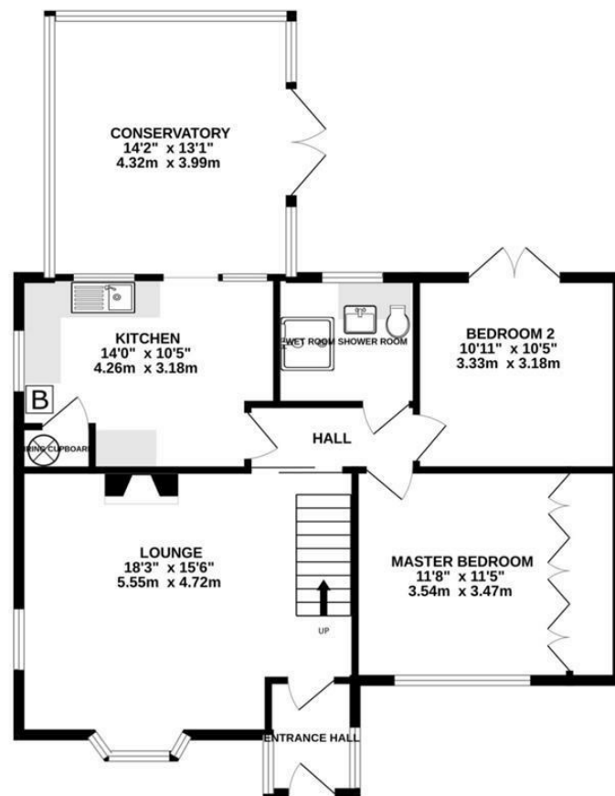
GROUND FLOOR 962 sq.ft. (89.3 sq.m.) approx.
