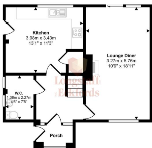
Ground Floor Approx 45 sq m / 488 sq ft
