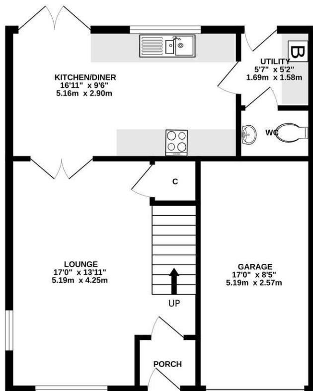
GROUND FLOOR 594 sq.ft. (55.2 sq.m.) approx.
