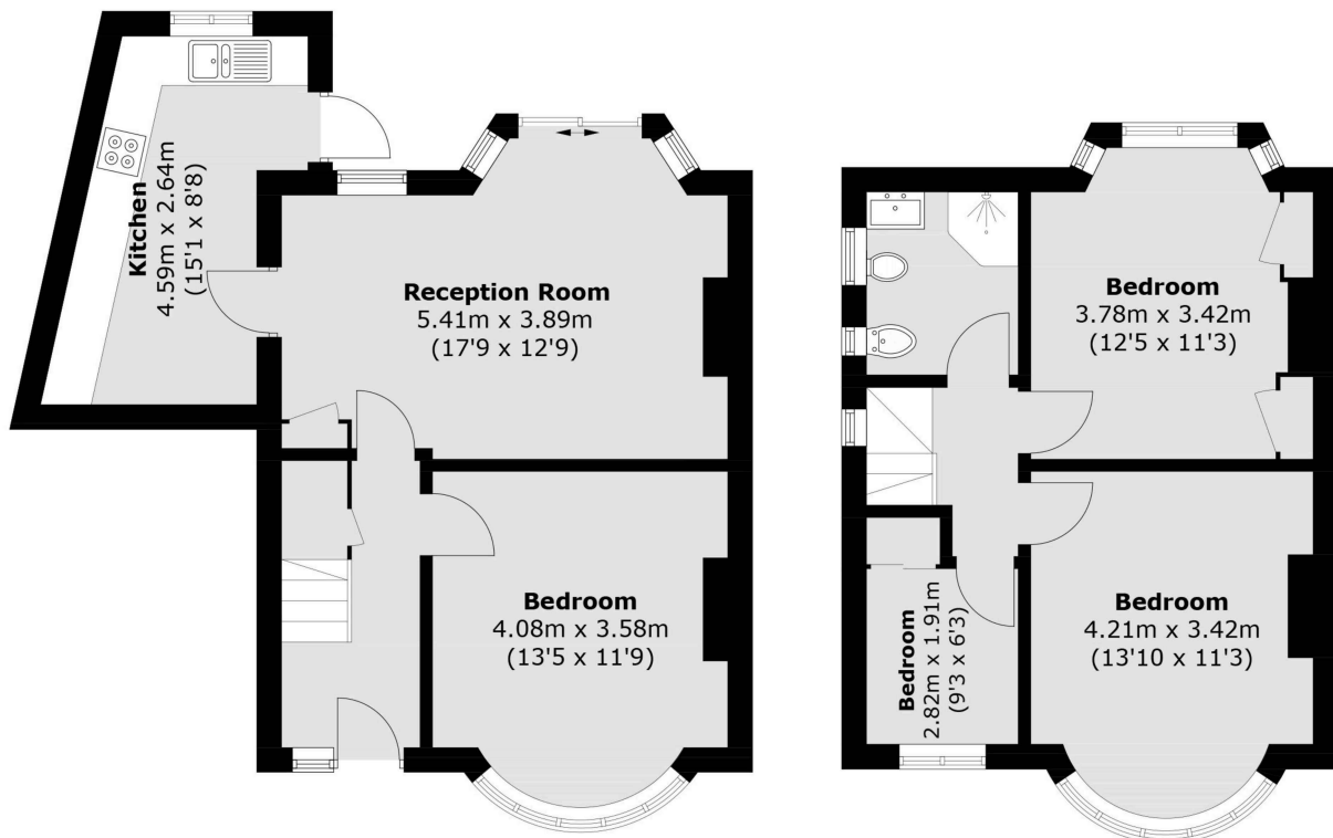
Ground Floor
