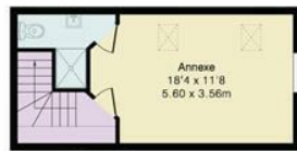
Garage First Floor
