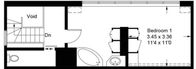
First Floor
