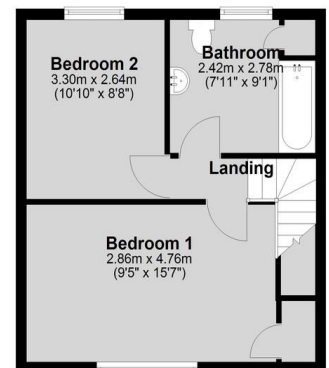
First Floor Approx. 34.5 sq. metres (371.1 sq. feet)
