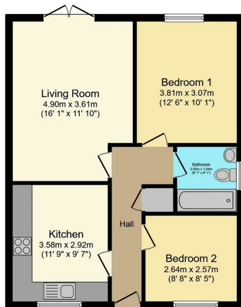
Floor Plan
