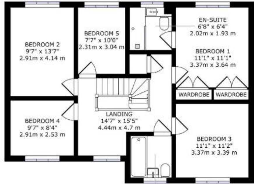
1st FLOOR
