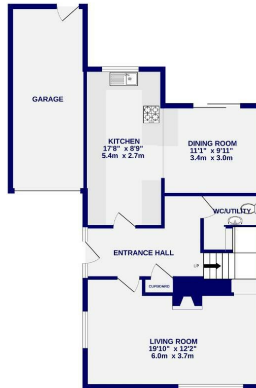
GROUND FLOOR 819 sq.ft. (76.1 sq.m.) approx.
