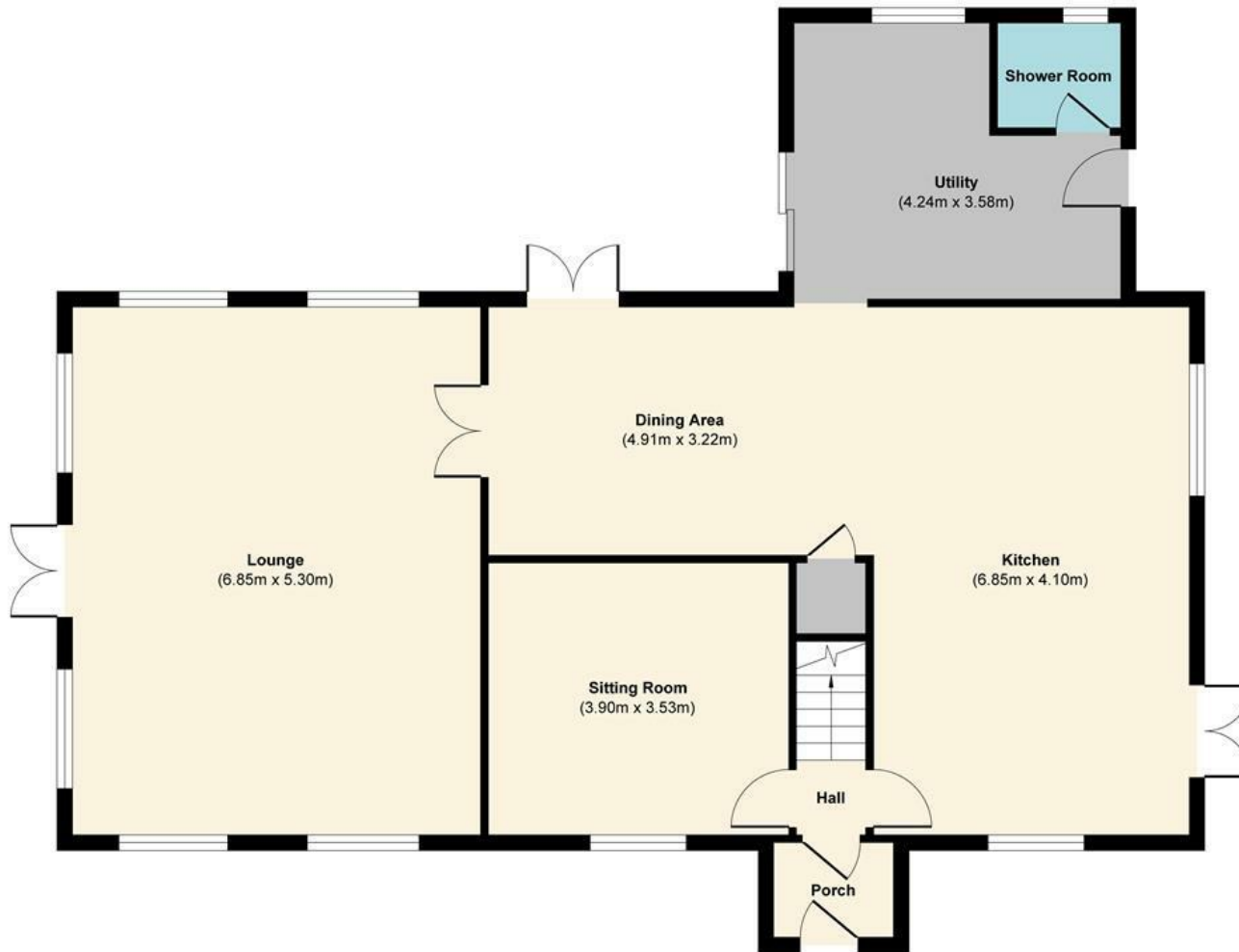
Ground Floor Approximate Floor Area (115.30 sq. m)
