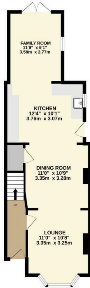
GROUND FLOOR 551 sq.ft. (51.2 sq.m.) approx.
