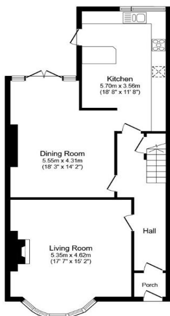
Ground Floor Floor area 79.2 sq.m. (852 sq.ft.)
