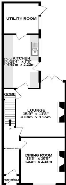
GROUND FLOOR 504 sq.ft. (46.2 sq.m.) approx.
