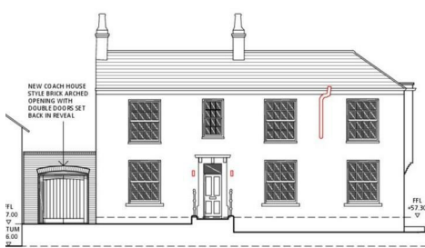
NORTH EAST ELEVATION
