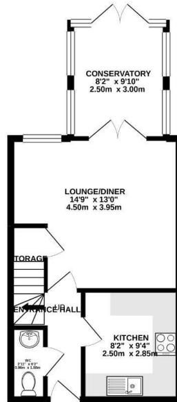
GROUND FLOOR 403 sq.ft. (37.4 sq.m.) approx.
