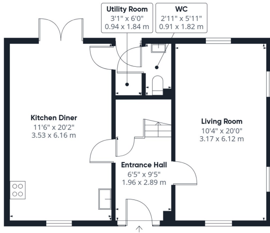
Floor 0 Building 1
