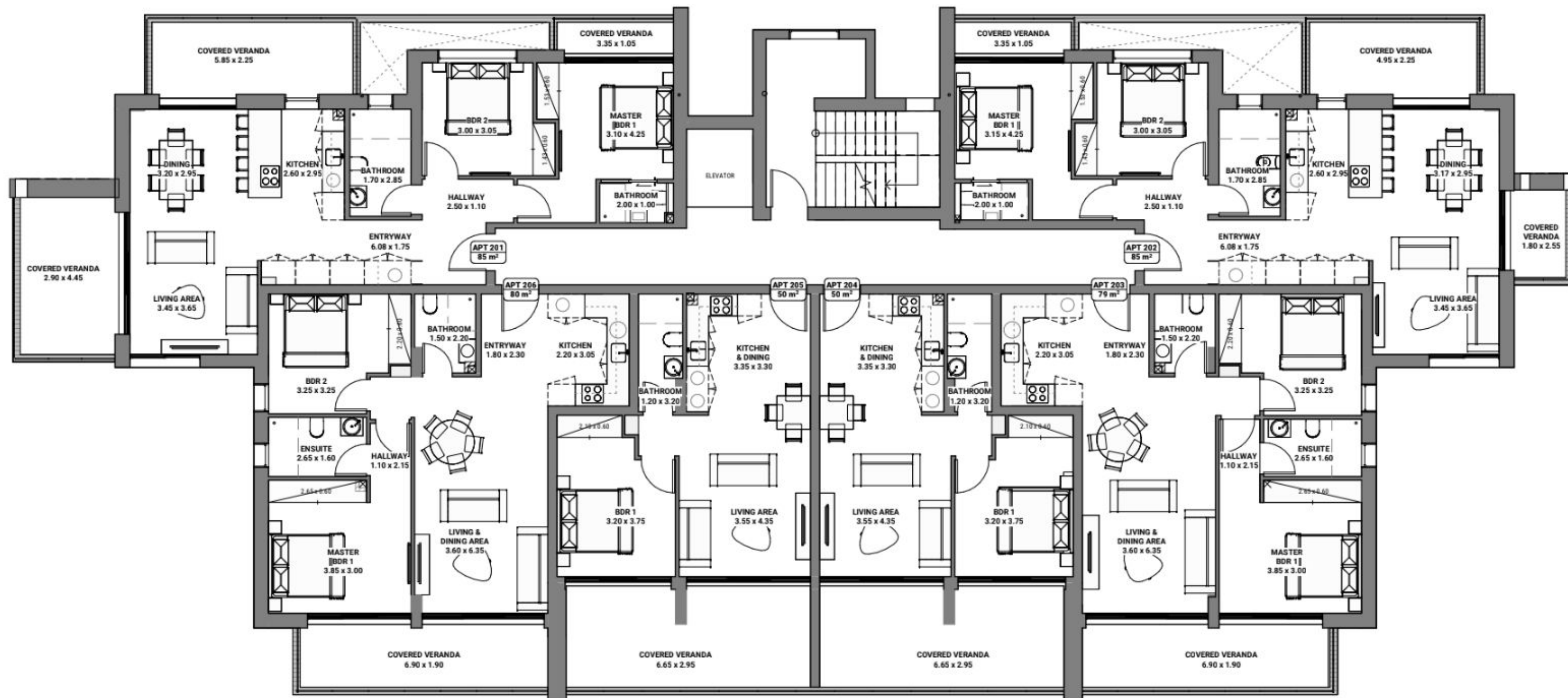
1 Brochure-Second Floor Plan 1 : 100
