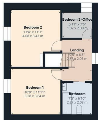
Floor 2
