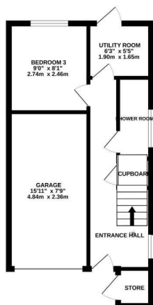
GROUND FLOOR 372 sq.ft. (34.5 sq.m.) approx.
