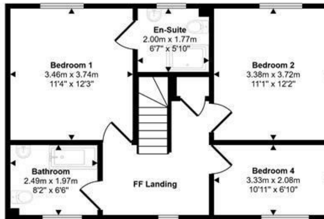
First Floor Approx 54 sq m / 581 sq ft
