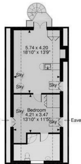
First Floor Above Garage
