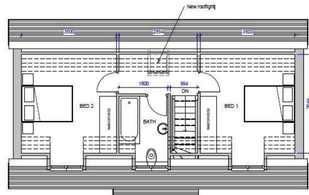
2 First Floor 1:50
