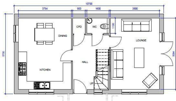
1 Ground Floor 1:50
