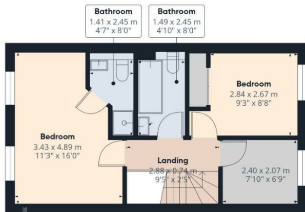
Floor 2
