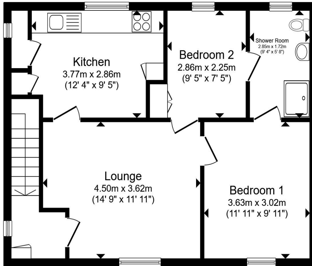
First Floor
