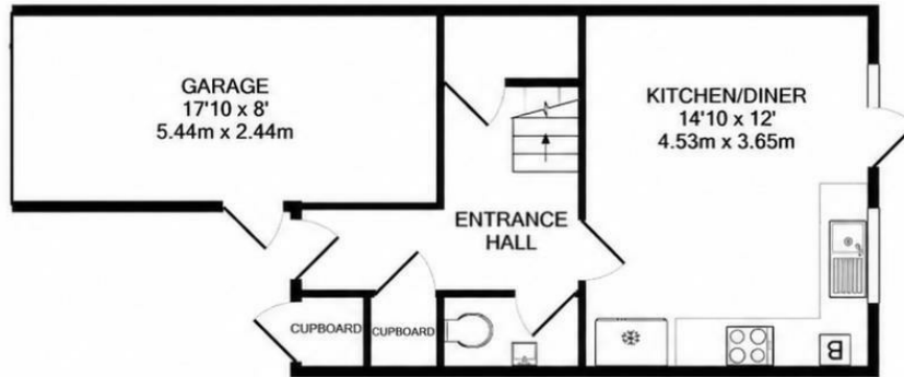
GROUND FLOOR APPROX. FLOOR AREA 452 SQ.FT. (42.0 SQ.M.)
