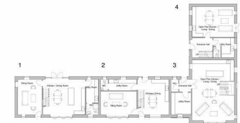
1 Ground Floor 1 : 100
