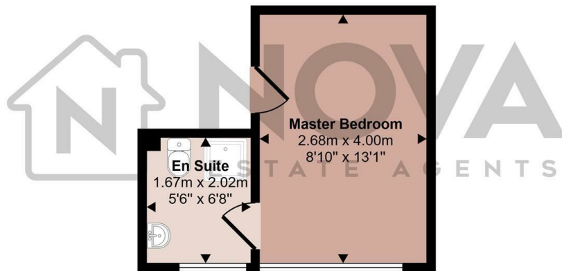
First Floor
