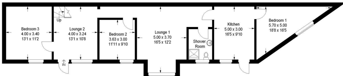
Ground Floor
