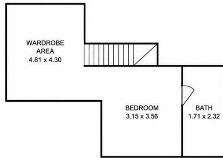
FLOOR PLAN UPPER FLOOR
