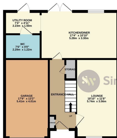
GROUND FLOOR 578 sq.ft. (53.7 sq.m.) approx.
