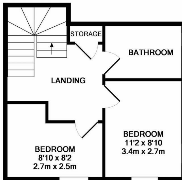
1ST FLOOR
