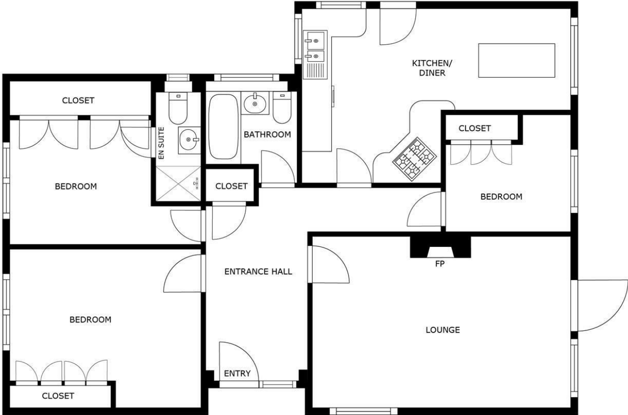
FLOOR PLAN
