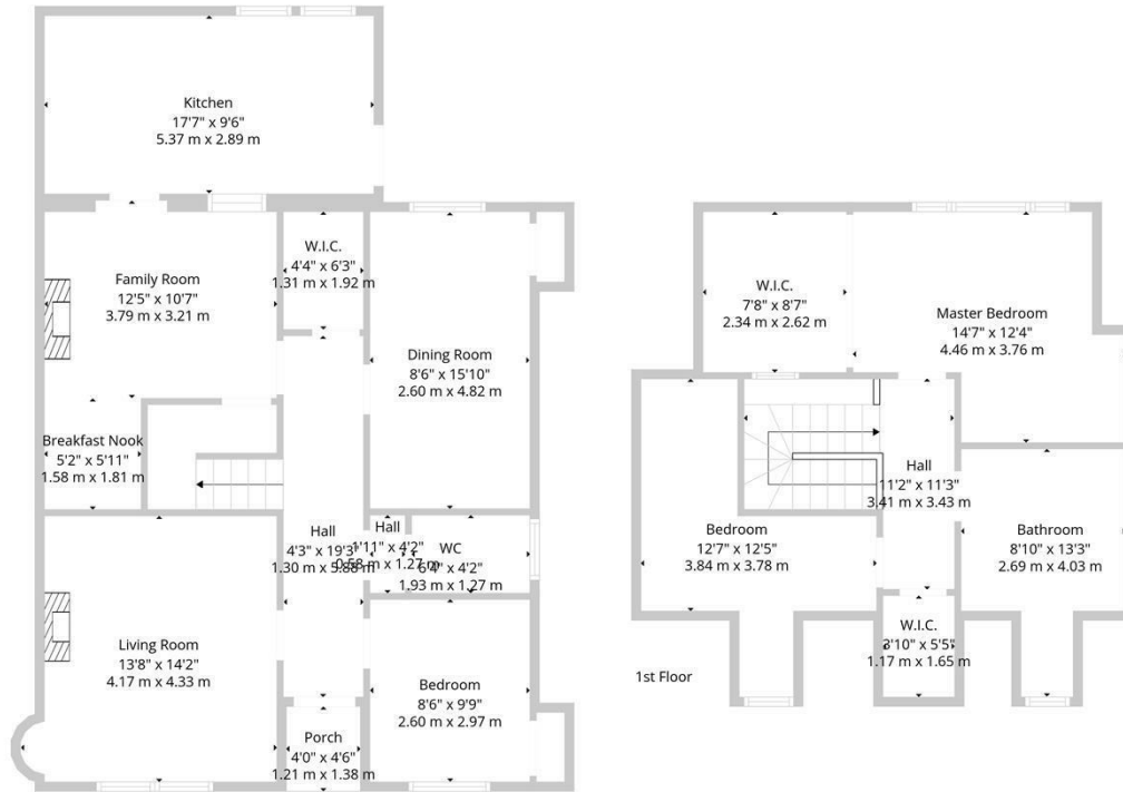
Ground Floor
