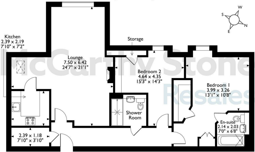
Second Floor The position & size of doors, windows, appliances and other features are approximate only. © ehouse. Unauthorised reproduction prohibited. Drawing ref. dig/8679179/DST.
