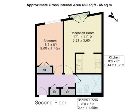
Floor Plan
