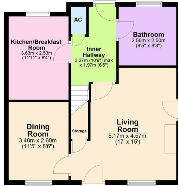
Ground Floor Approx. 53.9 sq. metres (579.8 sq. feet)
