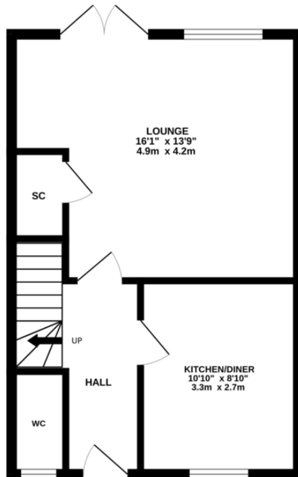
GROUND FLOOR 396 sq.ft. (36.8 sq.m.) approx.
