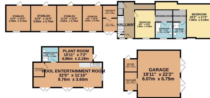
GROUND FLOOR 2465 sq.ft. (229.0 sq.m.) approx.
