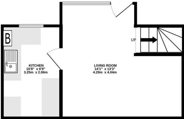
GROUND FLOOR 244 sq.ft. (22.7 sq.m.) approx.
