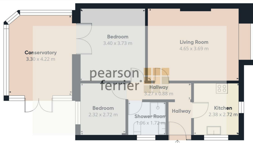
Floor 0 Building 1
