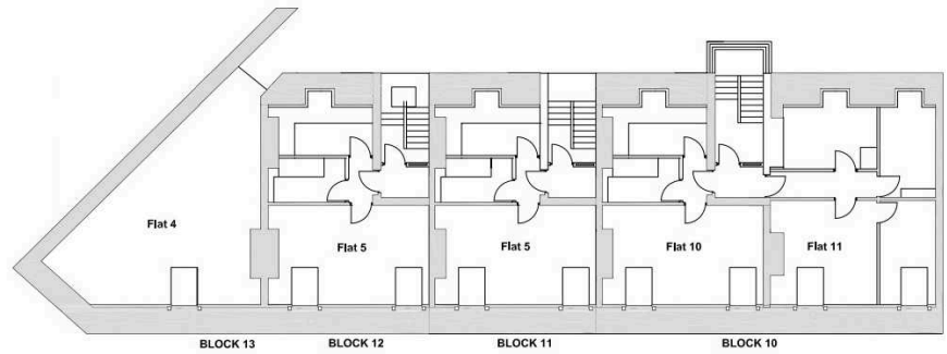
THIRD FLOOR
